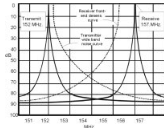
Figure 2 Band Pass Duplexer Response
