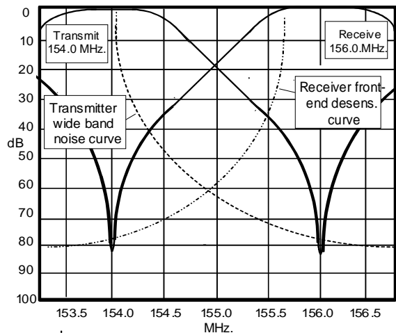
Figure 4 Pass/Reject Duplexer Response Curves
